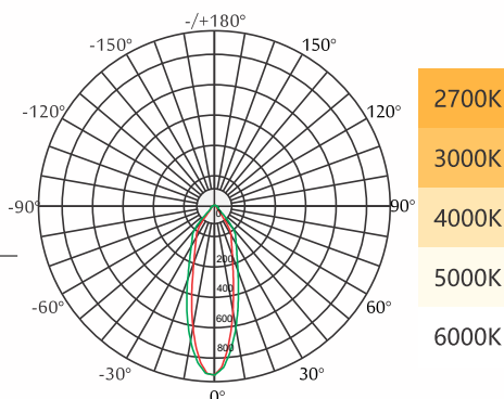
Beam Angle
