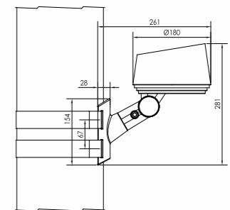
AVL Dia of pole(168-268)mm
